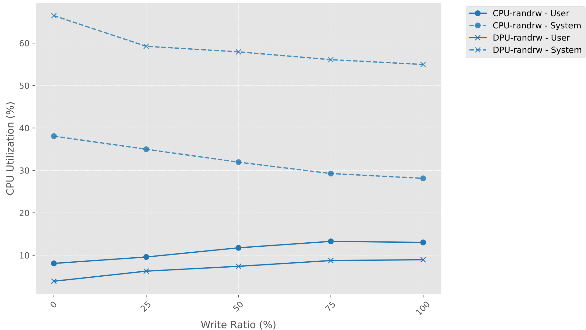
CPU Utilization vs Write Ratio (rwmixwrite-64k)
